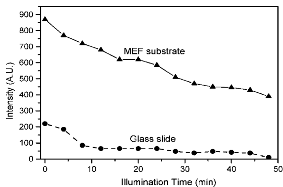
Fig. 5. Photo stability of the SNAFL-2-Dextran (pH 6.3) immobilized on the MEF substrate (SiFs) and glass (control sample). The illumination conditions were identical for the both samples, green LED, 535 mW, and 0.5 mW.
