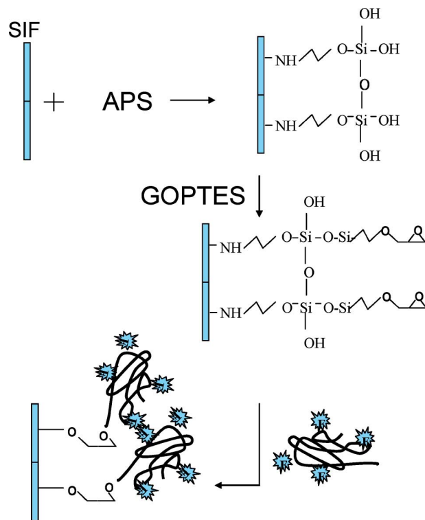
Fig. 2. Experimental procedure for the immobilization of the pH probe onto SiFs (silver island films).
