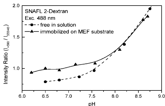
Fig. 4. The pH sensitivity of SNAFL-2 is retained in the presence of silver nanoparticles. The intensity on the MEF substrate is about 30–40 times brighter than the intensity of probe immobilized on glass slides. The ratios however are similar.
