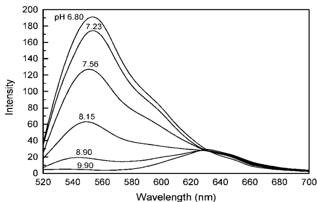
Fig. 3. Emission spectra of SNAFL-2-Dextran in solution in various pH buffers (PBS buffer), with 130 mM KCl. The excitation wavelength was 488 nm and temperature 23°C.
